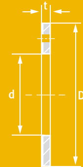
TFA/P Thrust washer
